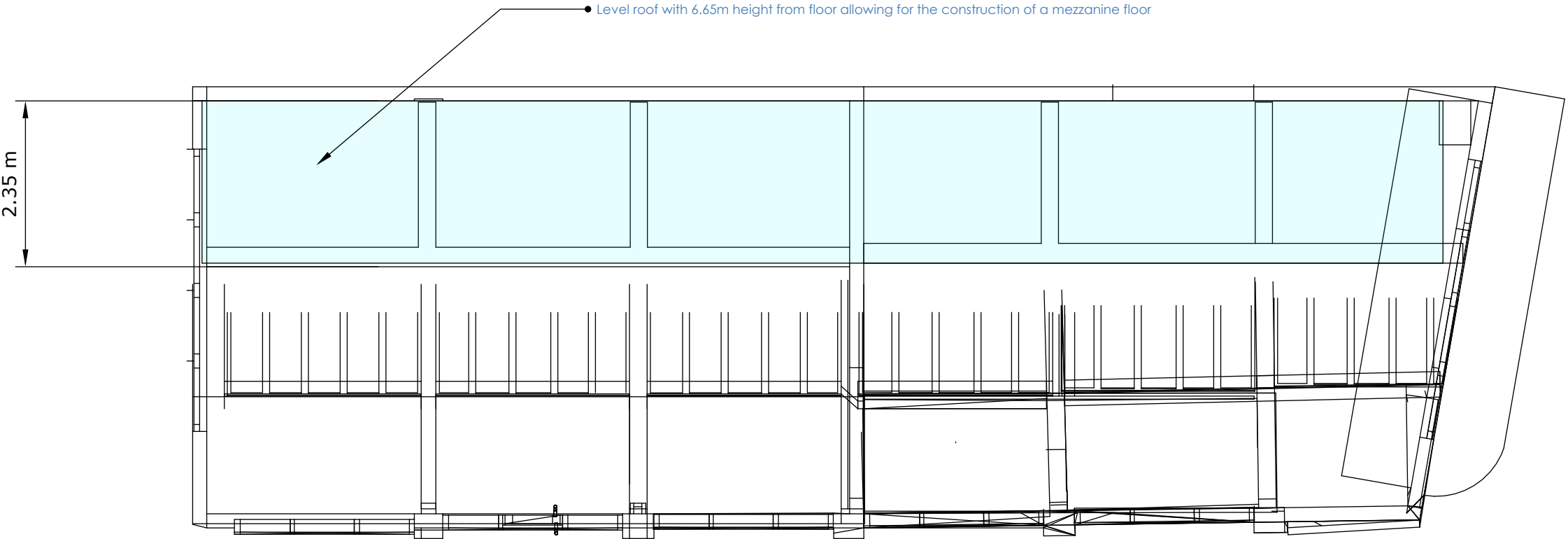
Ceiling Plan
